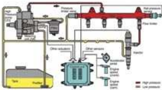
“Common Rail” Doosan DLo8 Engine
